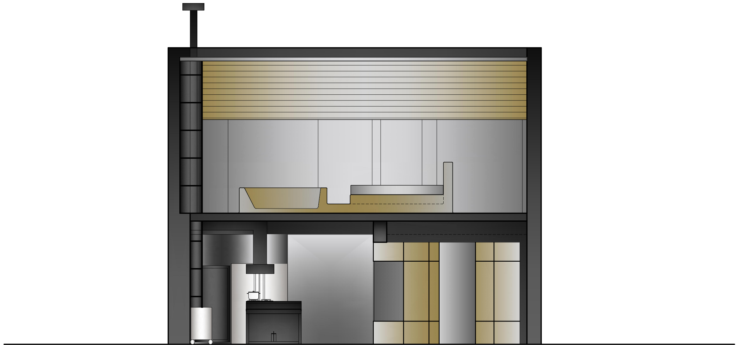
C-C SECTION
